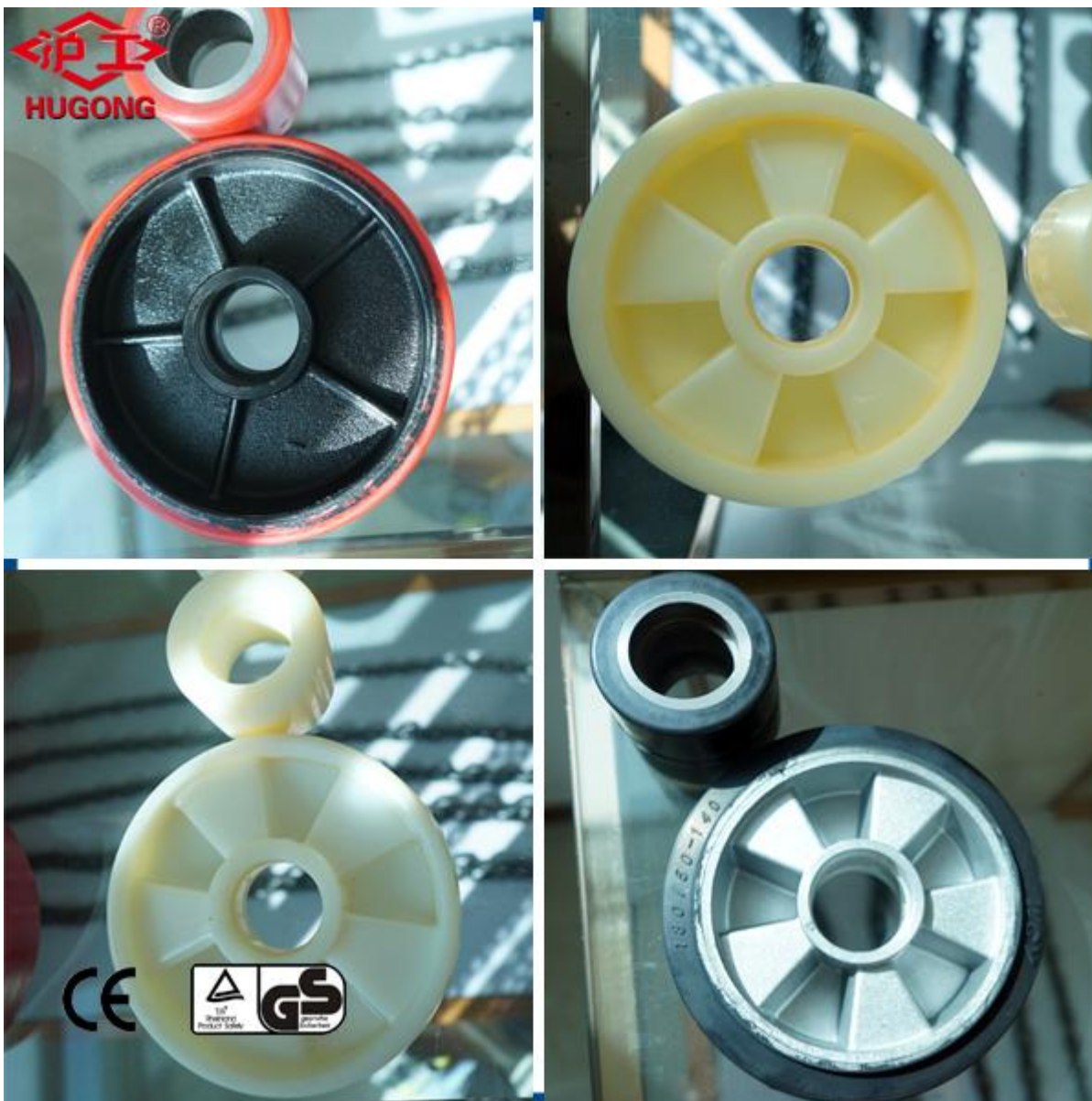
5. heavy duty pallet jack Rocker arm widened and thickened can ensure the long life.
